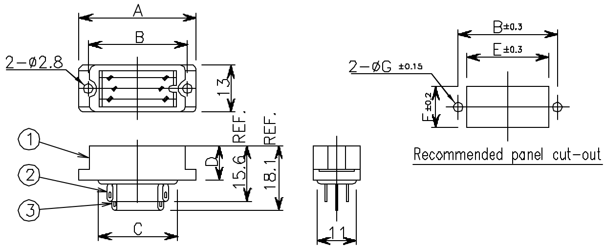
Contact arrangement for 8, 16, 20, 25, 34, 50 pos.
