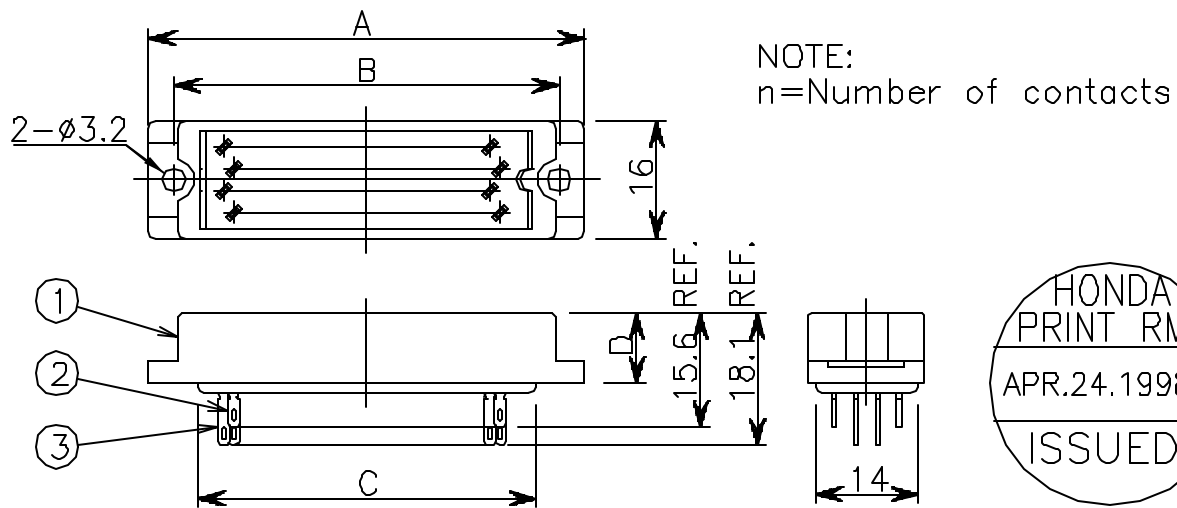
Contact arrangement for 60 pos.
