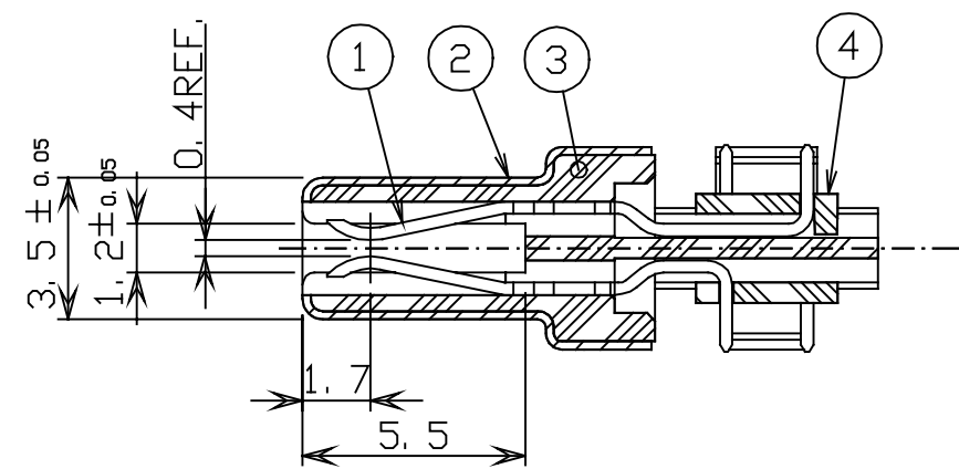
CONTACT DETAIL(5/1)
